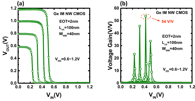
Fig. 16. (a) V_{OUT} versus V_{IN} of a 100-nm L_{ch} , 40-nm W_{NW} , and 2-nm EOT Ge IM NW CMOS inverter with (b) highest voltage gain of 54 V/V.
