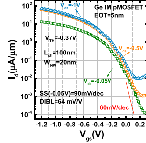
Fig. 11. Transfer curves of a 100-nm L_{ch} and 20-nm W_{NW} Ge IM NW pMOSFET with an EOT of 5 nm.
