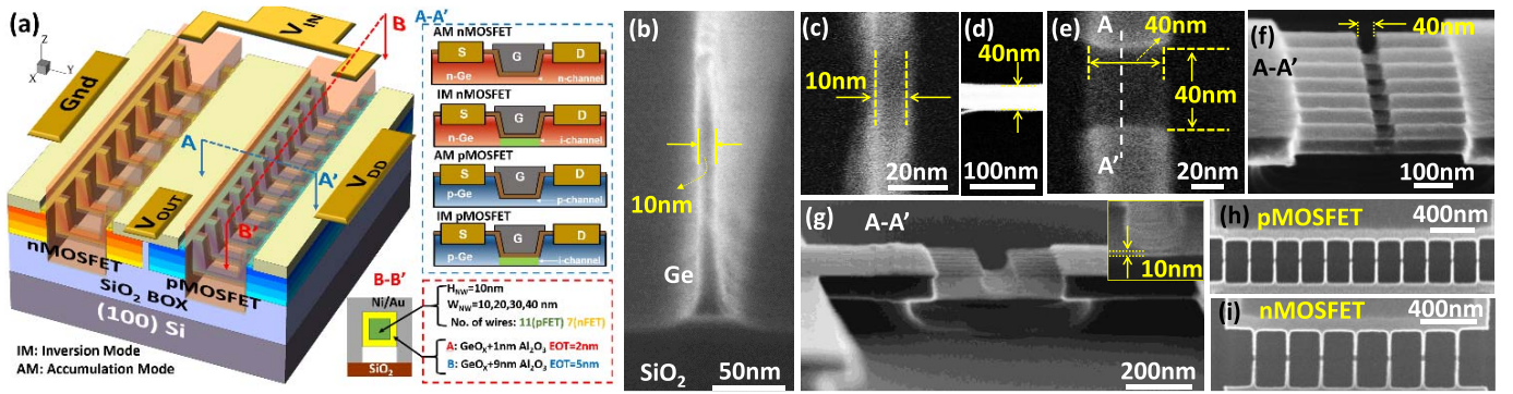
Fig. 2. (a) Device 3-D schematic and key geometry parameters of the Ge NW CMOS. Cross-sectional schematics of the NW CMOS in parallel (A-A') and perpendicular (B-B') to the NW direction with four types of operation modes (AM and IM nMOSFETs, AM and IM pMOSFETs) are listed. (b)–(i) SEM images of various structures on Ge: (b) Titled image of one of the narrowest fin structures with W_{FIN} = 10\text{nm} and an aspect ratio of 18. (c) Top-down image of the narrowest NW with 10\text{-nm } W_{NW} . (d) ZEP e-beam resist mask to define the smallest channel length of 40\text{nm} in the IM devices. (e) NW with 40\text{-nm } W_{NW} and 40\text{-nm } L_{ch} . The darker area on the NW is the recessed region with reduced NW height. (f) Freestanding NWs with 40\text{-nm } L_{ch} . (g) Zoomed-in of the Ge NWs (inset: H_{NW} of 10\text{nm} ). (h) and (i) NWs in the channel areas of p- and nMOSFETs for CMOS integration.
