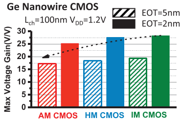
Fig. 17. Maximum voltage of the Ge NW CMOS inverters with different operation modes and EOTs.
