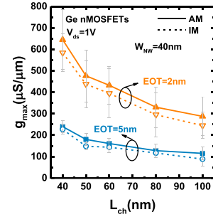
Fig. 10. g_{max} scaling metrics of the AM and IM Ge NW nMOSFETs with an EOT of 2 and 5 nm. AM and smaller EOT devices have larger g_{max} .
