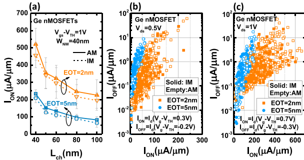
Fig. 9. (a) I_{ON} scaling metrics of the AM and IM Ge NW nMOSFETs with the EOTs of 2 and 5 nm. AM and smaller EOT devices have larger I_{ON} . (b) I_{OFF} versus I_{ON} of the AM and IM Ge nMOSFETs with L_{ch} from 100 to 40 nm and different EOTs at low V_{DD} of 0.5 V. (c) I_{OFF} versus I_{ON} of the Ge AM and IM nMOSFETs with L_{ch} from 100 to 40 nm and different EOTs at high V_{DD} of 1 V.
