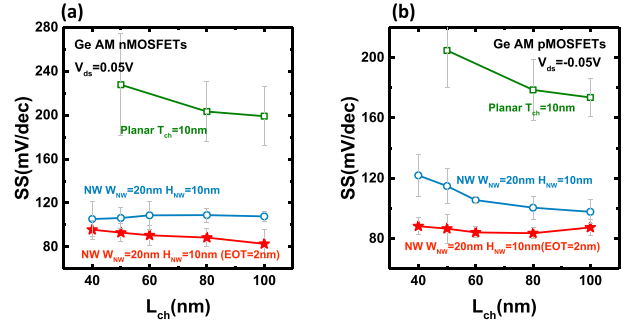
Fig. 19. SS versus L_{ch} of the Ge NW MOSFETs with different EOTs and planar MOSFETs at low V_{ds} of \pm 0.05 V. (a) AM nMOSFETs. (b) AM pMOSFETs.
