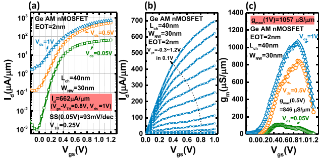
Fig. 8. (a) Transfer curves of a 40-nm L_{ch} , 30-nm W_{NW} , and 2-nm EOT Ge AM NW nMOSFET with I_{ON} of 662 \mu A/\mu m at V_{ds} of 1 V and V_{gs} - V_{TH} = 0.8 V. (b) Output curves of the same device in (a). The I_{max} is \sim 700 \mu A/\mu m . (c) g_m versus V_{gs} curves of the same device given in (a). Record high g_{max} of 1057 \mu S/\mu m is obtained.
