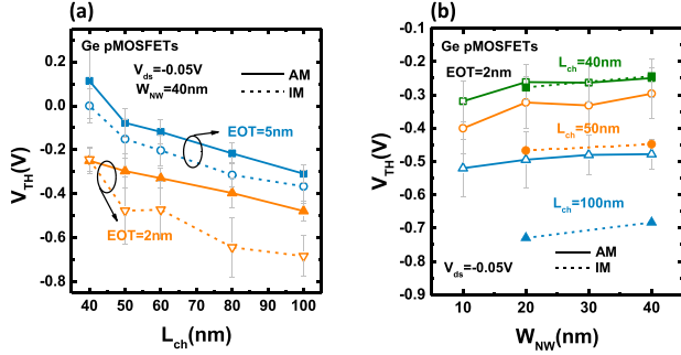
Fig. 12. (a) V_{TH} scaling metrics of the AM and IM Ge NW pMOSFETs with an EOT of 2 and 5 nm and W_{NW} of 40 nm. IM and thinner EOT pMOSFETs have larger V_{TH} . (b) W_{NW} dependence of the V_{TH} of the AM and IM Ge NW pMOSFETs with an EOT of 2 nm. Smaller W_{NW} devices have larger V_{TH} .
