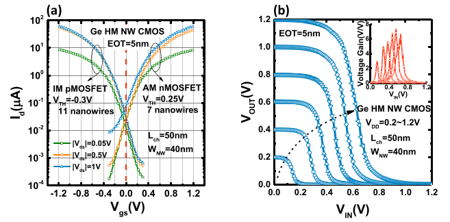
Fig. 15. (a) I_d - V_{gs} of the AM nMOSFET and the IM pMOSFET inside a 50-nm L_{ch} and 40-nm W_{NW} hybrid Ge NW CMOS inverter with a 5-nm EOT. The two show symmetrical performance. (b) V_{OUT} versus V_{IN} of the same CMOS inverter shown in (a). Inset: voltage gain.
