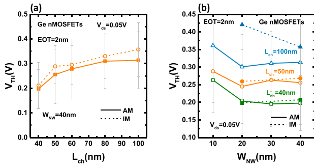
Fig. 5. (a) V_{TH} scaling metrics of the Ge NW nMOSFETs with an EOT of 2 nm and 40-nm W_{NW} . IM and longer L_{ch} nMOSFETs have larger V_{TH} . (b) W_{NW} dependence of the V_{TH} of the AM and IM Ge NW nMOSFETs with an EOT of 2 nm. Smaller W_{NW} devices have larger V_{TH} .
