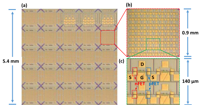
Fig. 3. (a) Top-down view of a fabricated chip under the optic microscope. The size parameters of the chip are marked. (b) Enlargement of one die inside the chip [red square in (a)]. (c) Zoomed-in view of Ge CMOS devices array [green square in (b)].
