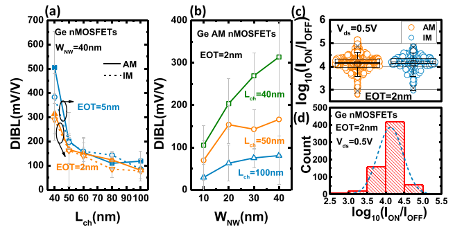
Fig. 7. (a) DIBL scaling metrics of the AM and IM Ge NW nMOSFETs with an EOT of 2 and 5 nm and W_{NW} of 40 nm. IM and smaller EOT devices have better DIBL. (b) W_{NW} dependence of the DIBL of the AM Ge NW nMOSFETs with an EOT of 2 nm. Smaller W_{NW} devices have better DIBL. (c) and (d) BOX plot and histogram of the I_{ON}/I_{OFF} of the Ge NW nMOSFETs with the EOTs of 2 nm at V_{ds} of 0.5 V based on more than 800 measured data points.
