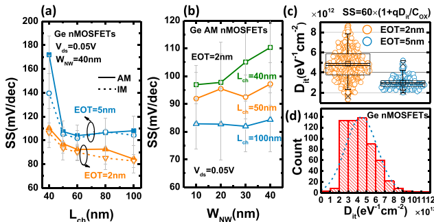
Fig. 6. (a) SS scaling metrics of the AM and IM Ge NW nMOSFETs with an EOT of 2 and 5 nm and W_{NW} of 40 nm. IM and smaller EOT devices have better SS. (b) W_{NW} dependence of the SS of the AM Ge NW nMOSFETs with an EOT of 2 nm. Smaller W_{NW} devices have better SS. (c) BOX plot for mid-gap D_{it} of Ge NW nMOSFETs with 2- and 5-nm EOT, extracted from SS based on more than 800 measured data points. (d) Histogram for mid-gap D_{it} .
