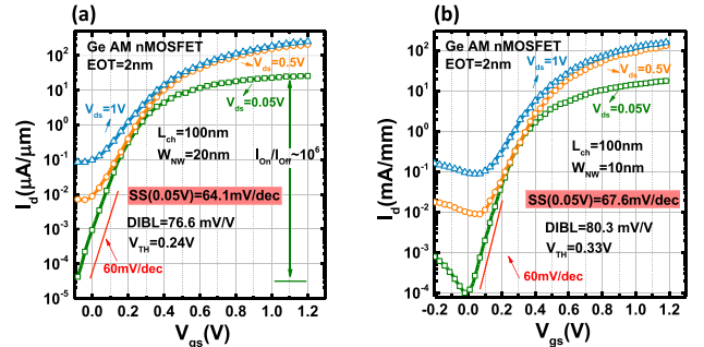
Fig. 4. (a) Transfer curves of a 100\text{-nm } L_{ch} and 20\text{-nm } W_{NW} Ge AM NW nMOSFET with SS = 64.1\text{mV/dec} at V_{ds} of 0.05\text{V} . (b) I_{ds} - V_{gs} curves of another device with sub-70 mV/dec SS at V_{ds} of 0.05\text{V} .
