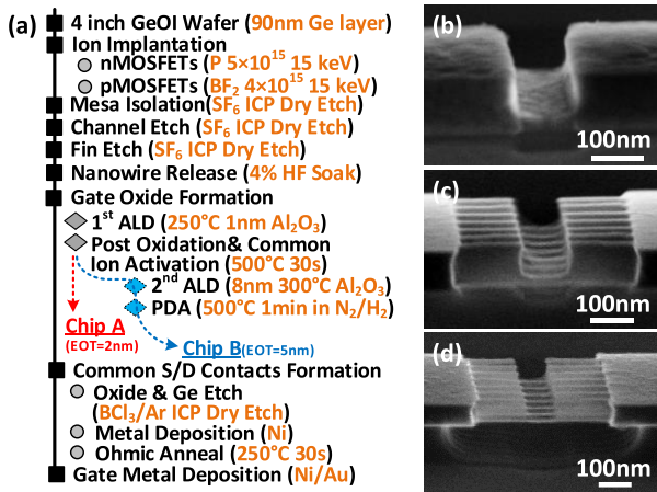
Fig. 1. (a) Fabrication process flow of the Ge NW CMOS. Devices with different gate oxide are fabricated in parallel. (b)–(d) Structure-wise evolution in the channel area: (b) Planar Ge recessed channel standing on the SiO 2 BOX layer. (c) 3-D Ge recessed fin channel standing on the SiO 2 BOX layer. (d) 3-D Ge freestanding recessed NW channel with the bottom SiO 2 removed.
