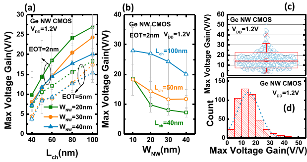
Fig. 18. (a) Maximum voltage gain scaling metrics of all the three types of Ge NW CMOS inverters with an EOT of 2 and 5 nm and W_{NW} of 20, 30, and 40 nm. Thinner EOT devices have larger voltage gain. (b) W_{NW} dependence of the maximum voltage gain of all the three types of Ge NW CMOS inverters with an EOT of 2 nm. Smaller W_{NW} devices have better values. (c) and (d) BOX plot and histogram for the maximum voltage gain of all the three types of Ge NW CMOS inverters at V_{DD} of 1.2 V based on more than 400 measured devices.
